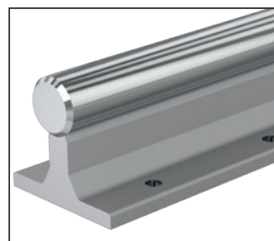
Steel shaft with shaft support rail, R1011
