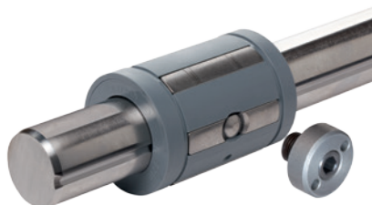
Type 1: One ball guide groove
