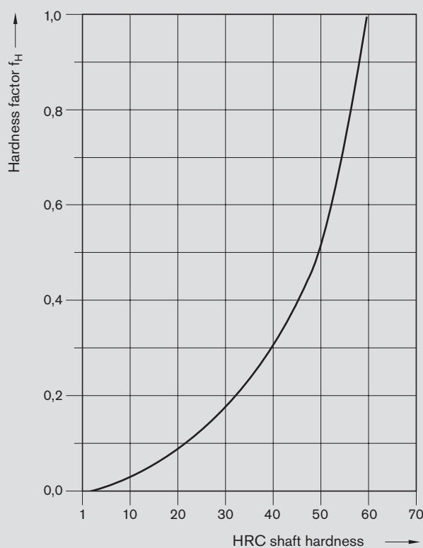
Diagram for hardness factor f_H
