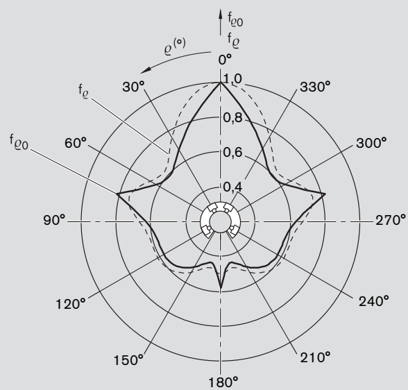
Shaft diameter 16
