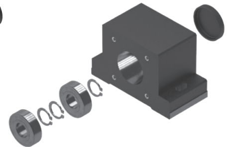
Pillow Block Unit SEC-L assembly
