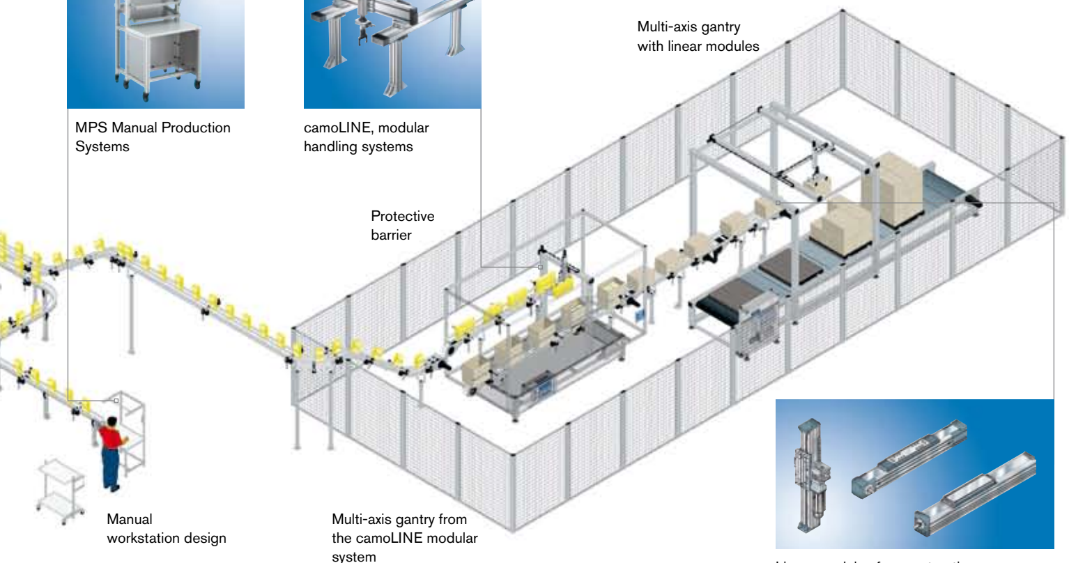
Linear modules for constructing multi-axis palletizing systems
